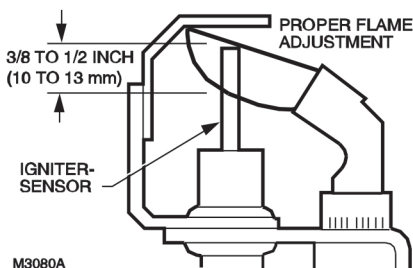
Figure 2. Proper flame adjustment
